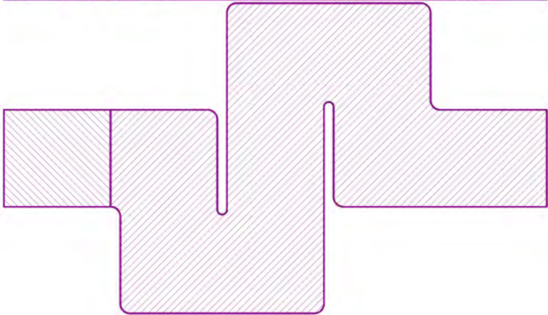
Fig. 2: Fill patterns in the “Flexible” and “Rigid” columns in the table identify the rigid and flexible areas of the board. 5
