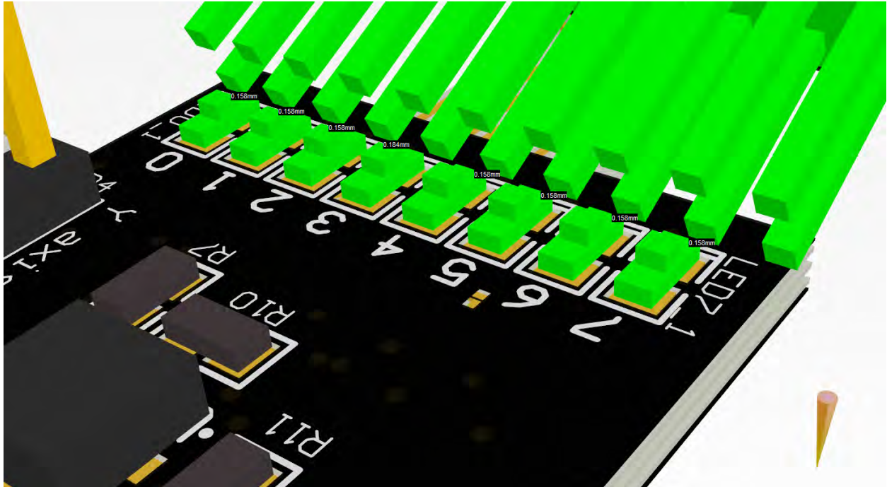
Fig. 5: Simulated bending of a flex circuit reveals a clearance violation between a flex-mounted pin-header and SMDs on the main rigid board. The violating components are highlighted green. 7
